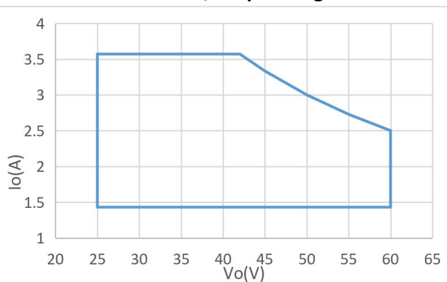
150PHL60CV I/V Operating Area
