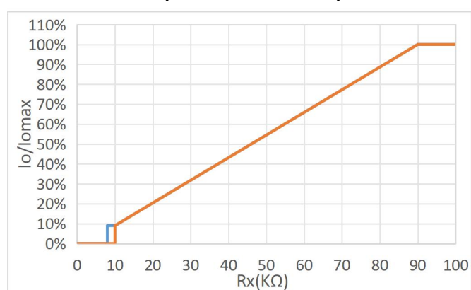
150PHL60CV-D0/150PHL180CV-D0 I_o/I_{omax} vs R_x
