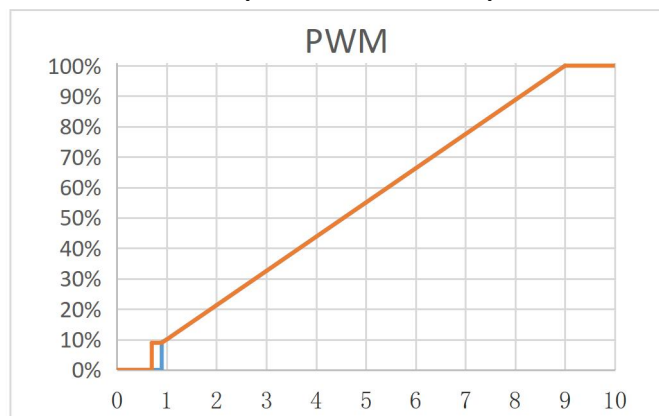
150PHL60CV-D0/150PHL180CV-D0 I_o/I_r vs V_{dim}
