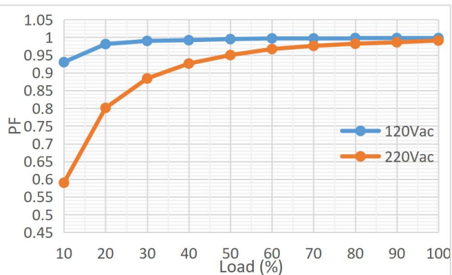
150PHL180CV Power Factor Vs Different Loads
