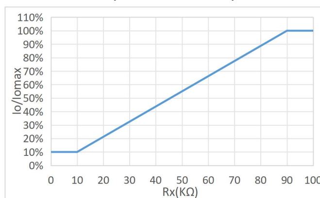
150PHL60CV-D1/150PHL180CV-D1 I_o/I_{omax} vs R_x
