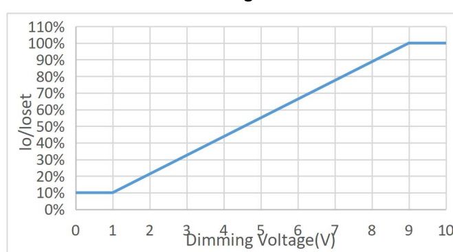
150PHL60CV-D1/150PHL180CV-D1 I_o/I_{oset} vs Dimming Voltage
