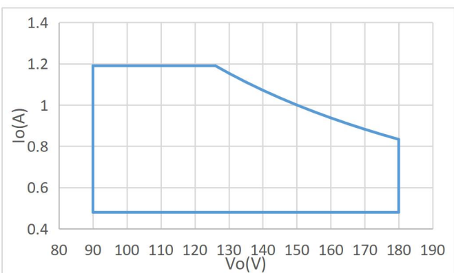
150PHL180CV I/V Operating Area
