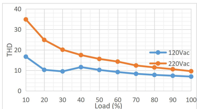
150PHL180CV Total Harmonics Vs Different Loads
