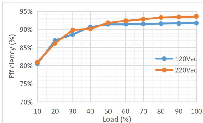
150PHL180CV Efficiency Vs Different Loads
