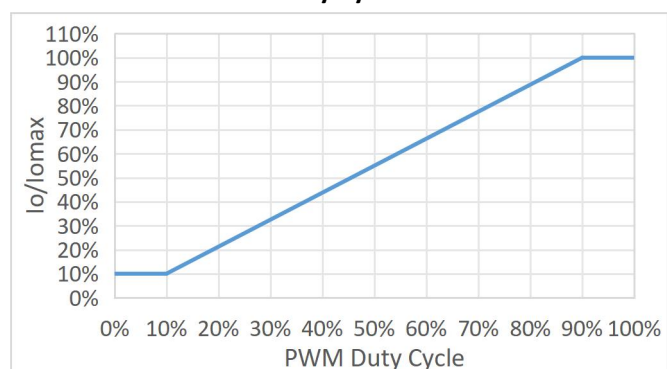
150PHL60CV-D1/150PHL180CV-D1 I_o/I_{omax} vs PWM Duty Cycle
