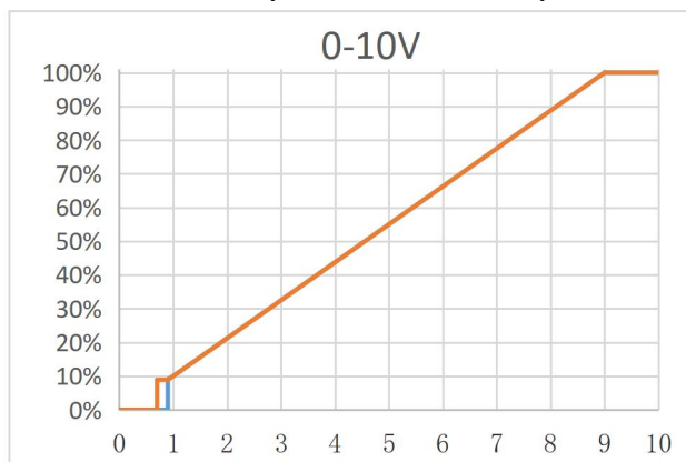
150PHL60CV-D0/150PHL180CV-D0 I_o/I_r vs V_{dim}
